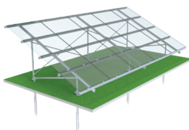
Material art. FV panel (optional) ANODIZED ALUMINIUM SOL-N-GROUND-SET 20
