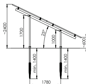
Material art. FV panel (optional) ANODIZED ALUMINIUM SOL-N-GROUND-SET 20
